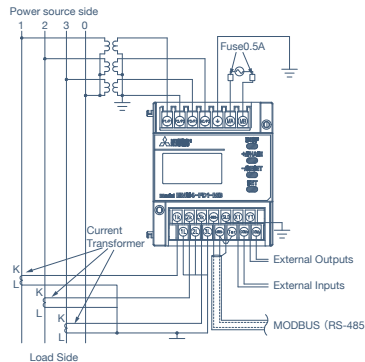
3P4W (with the voltage transformer)
