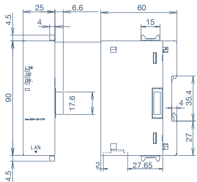
CC-Link IE field network Basic communication Unit (EMU4-CM-CIFB)
